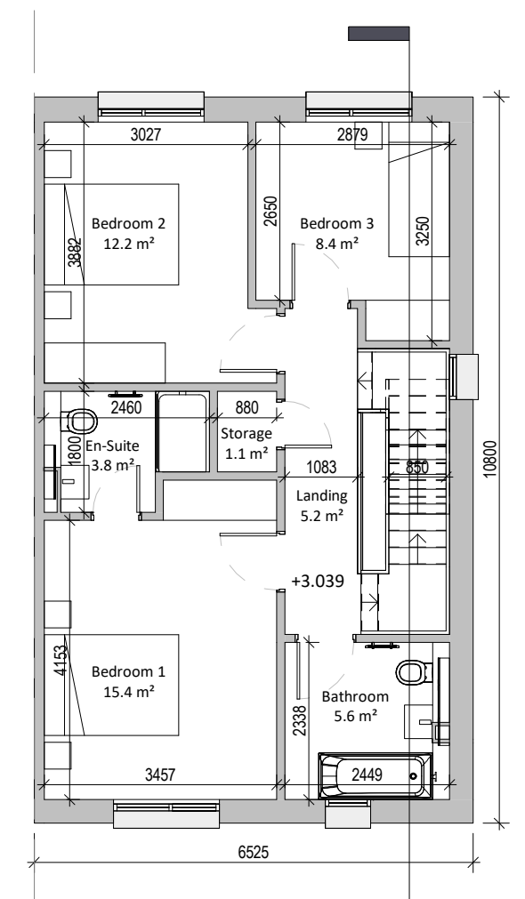
2 First Floor Plan 1 : 100
