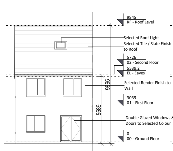
4 Rear Elevation 1 : 200
