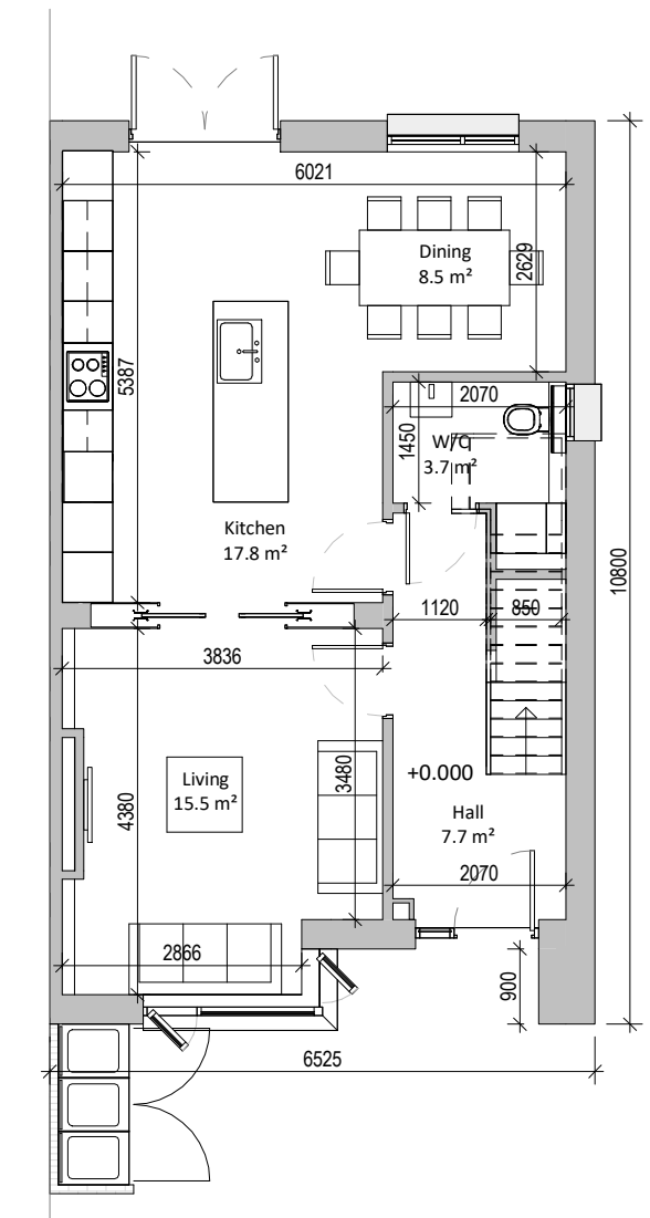
1 Ground Floor Plan 1 : 100
