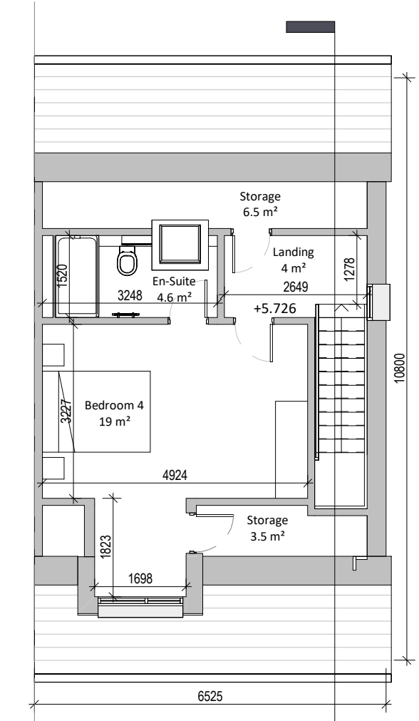
8 Second Floor Plan 1 : 100
