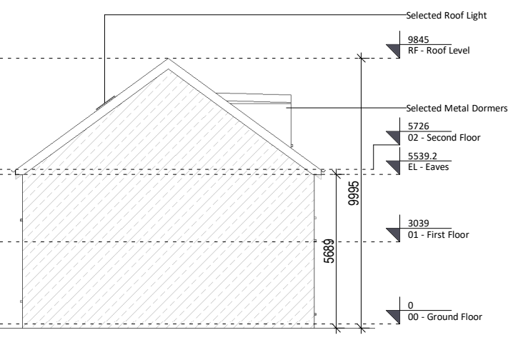
5 Left Elevation / Party Wall Section 1 : 200
